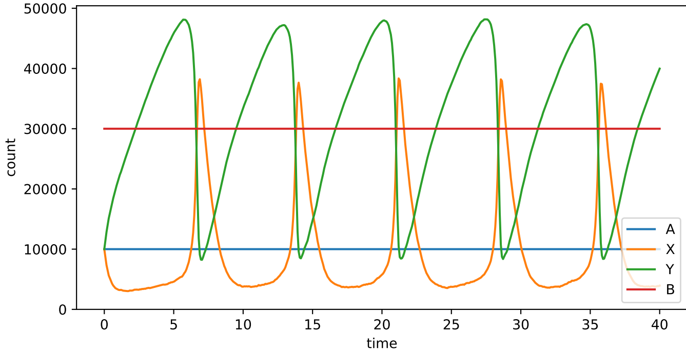
Order-3 Brusselator: batss, n=10^4
